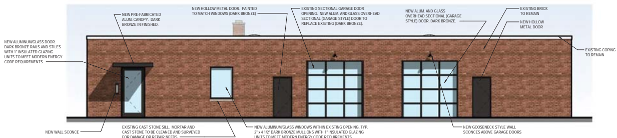
2 BUILDING EXTERIOR ELEVATION - WEST SCALE: 1/8" = 1'-0"
