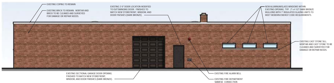
1 BUILDING EXTERIOR ELEVATION - EAST SCALE: 1/8" = 1'-0"
